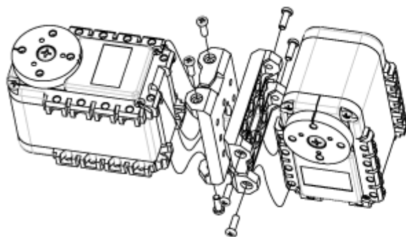
Exploded view
